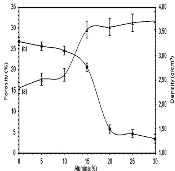
Fig. 4. Density (a) and porosity (b) of cordierite as a function of alumina addition.
