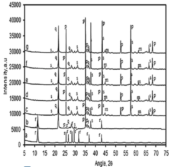
Fig. 1. The X-ray diffraction patterns of sintered samples at temperature of 1230 °C with different alumina content (a) 0, (b) 5, (c) 10, (d) 15, (e) 20, (f) 25, and (g) 30%. p = corundum, q = cristobalite, r = \alpha -cordierite, s = spinel, m = periclase.
