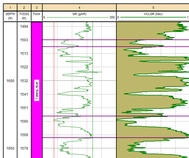
Gambar 18. Vsh interpretation
