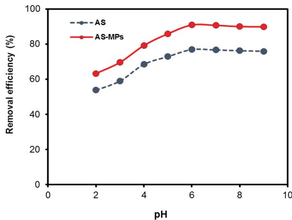
Fig. 6. Influence of pH on MB adsorption to AS and AS-MPs (contact time of 60 min, concentration of 100 mg L -1 , temperature of 27°C, and agitation speed of 100 rpm).
