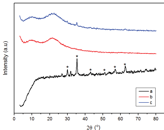
Fig. 2. XRD patterns of a) MPs, b) AS, and c) AS-MPs.
