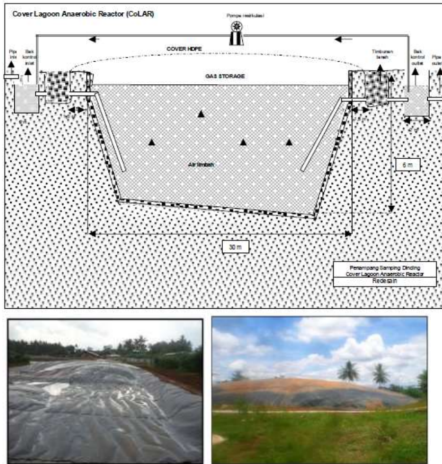
Figure 1.CoLAR design [21].
